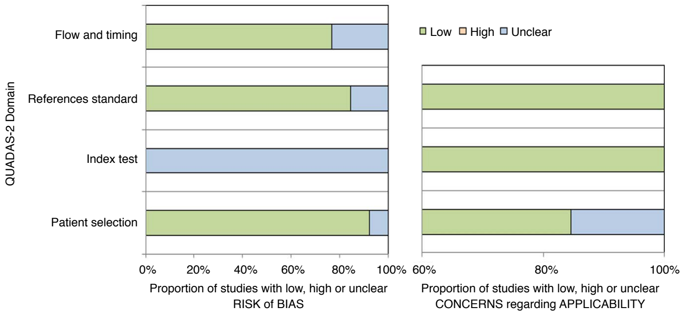
Supplementary Fig. 1. Quality assessment of the included studies based on the QUADAS-2 method.
