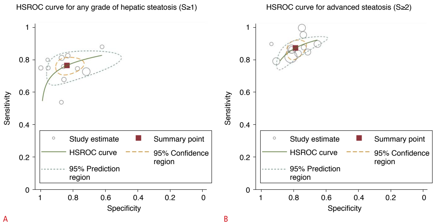
Supplementary Fig. 2. Hierarchical summary receiver operating characteristics (HSROC) curves. HSROC curves for any grade of hepatic steatosis ( S \geq 1 ) (A) and advanced steatosis ( S \geq 2 ) (B) are shown.
